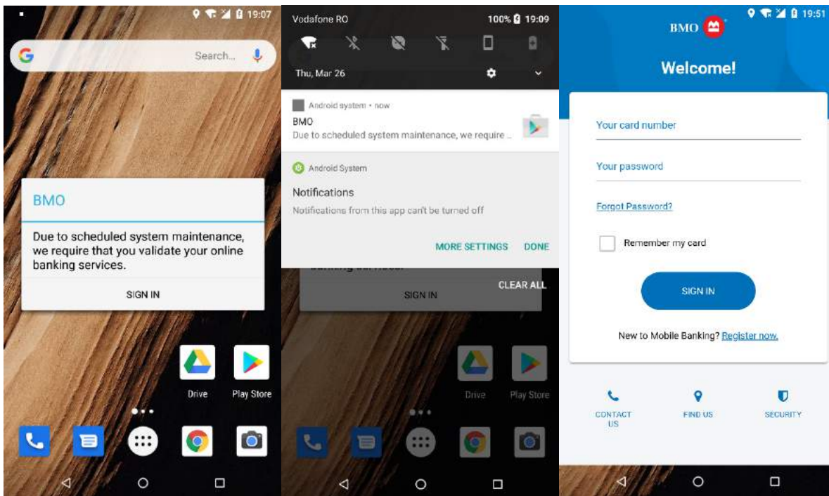
The dialog, notification, and page corresponding to the above command
